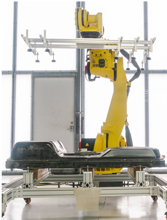
Battery pack disassembly
