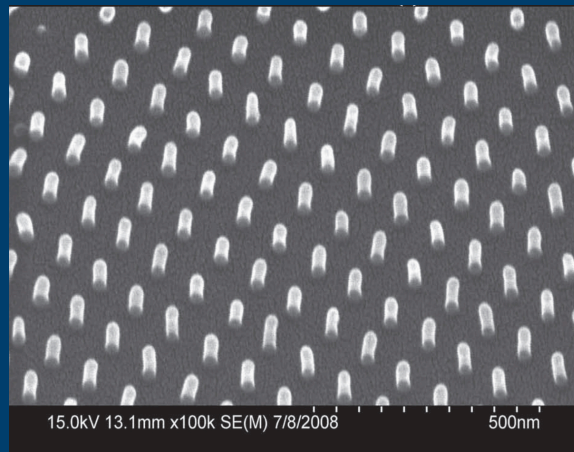
Electrode NanoArchitecture
