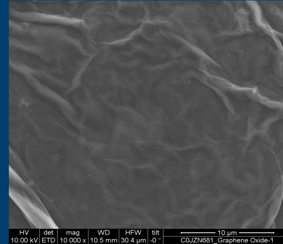
Graphene(s)
