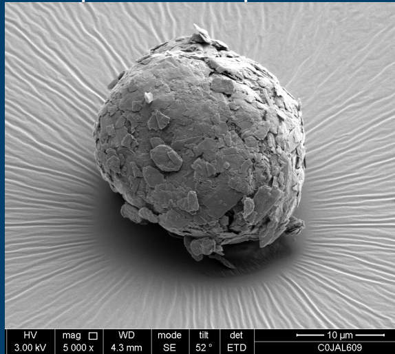
Spherical Graphite
