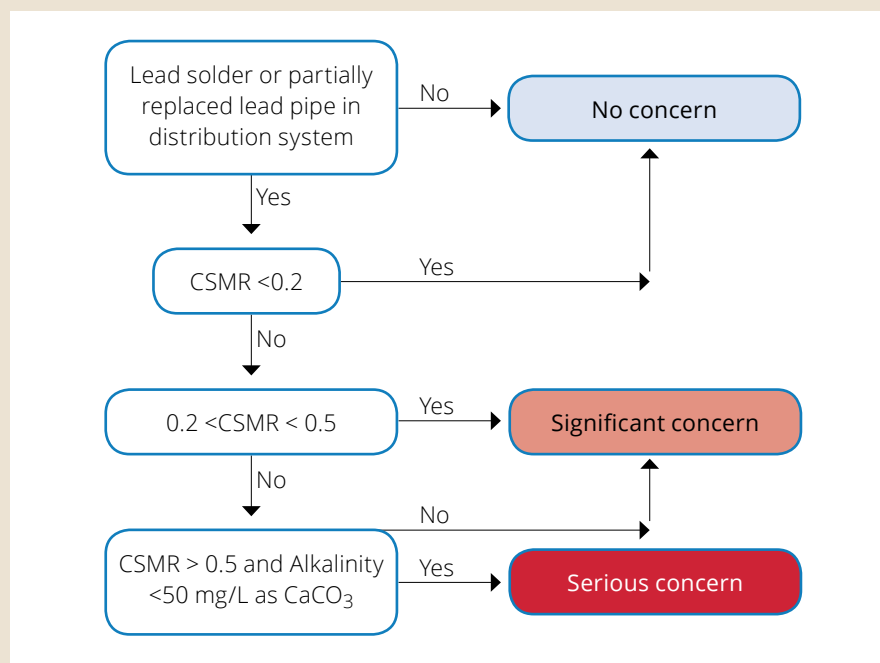
Figure 2 Decision Tool for assessing potential corrosion in lead pipes (from Nguyen, et al., 2010)
