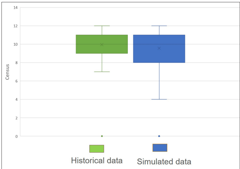
Figure 5: Model validation results (census comparison)
