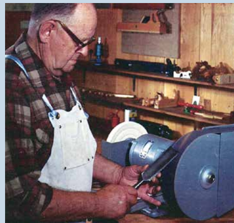
Woodcraft introduced the belt-buff concept 40 years ago with this Mark II system.
