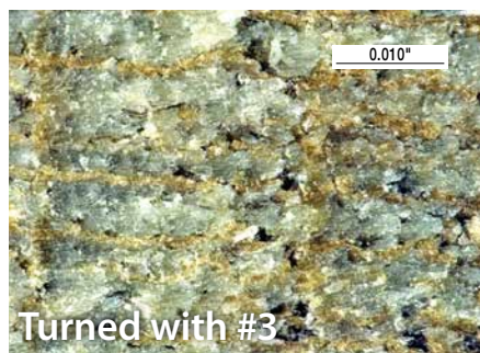
#3 Side View
