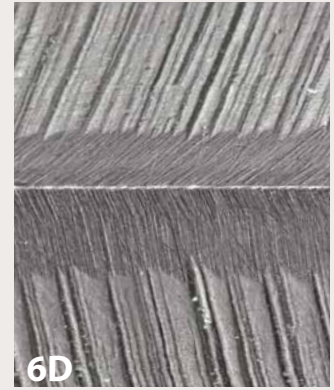
6D Edge view of skew chisel, ground and honed (200X).
