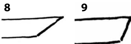
8. Conventional scraper bevel 9. Steeper bevel for finishing cuts
