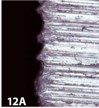
Cutting edge of a M2 HSS skew, ground (200X).
