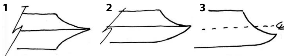
1. Conventional parting tool 2. Modified with convex edge 3. Ellsworth shop-made tool
