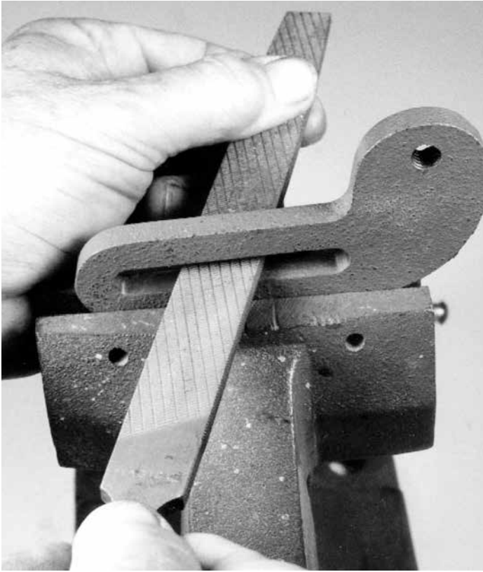
A file is used to open up the adjusting slot in the tool rest support. Also shown is the newly enlarged and threaded hole for the tool rest.
