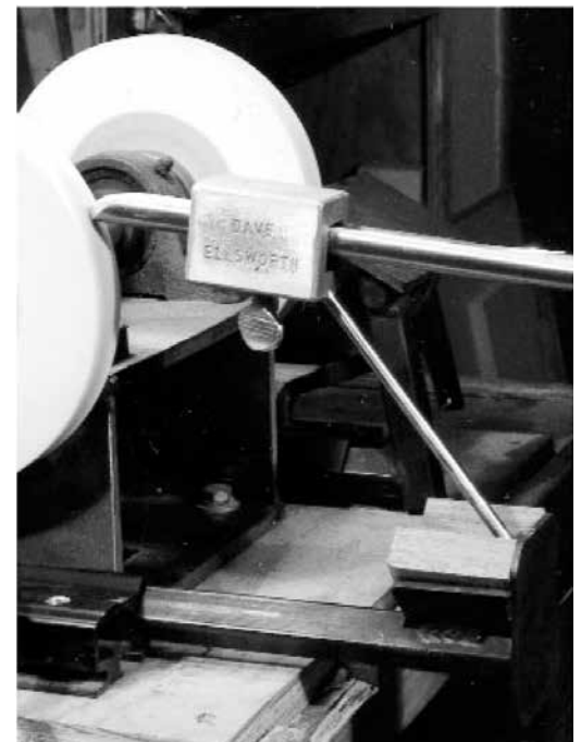
Ellsworth Jig
