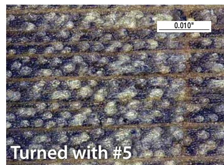
#5 Side View
